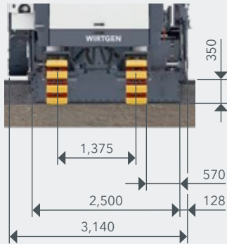
W 220 XF with 2.5 m milling drum assembly
