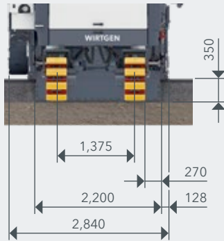
W 220 XF with 2.2 m milling drum assembly
