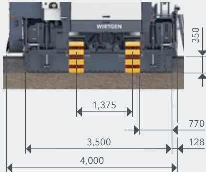
W 220 XF with 3.5 m milling drum assembly
