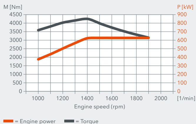
W 220 XF cold milling machine engine characteristics
