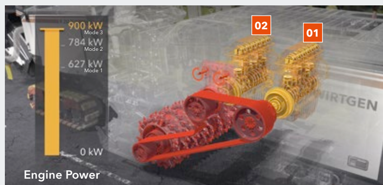
Engine characteristics of the cold milling machine W 250 XF
