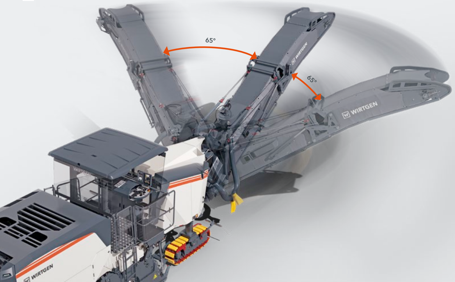
01 Increased scraper stroke for a wider range of milling applications and reduced wear. 02 The discharge conveyor has a large swing range.
