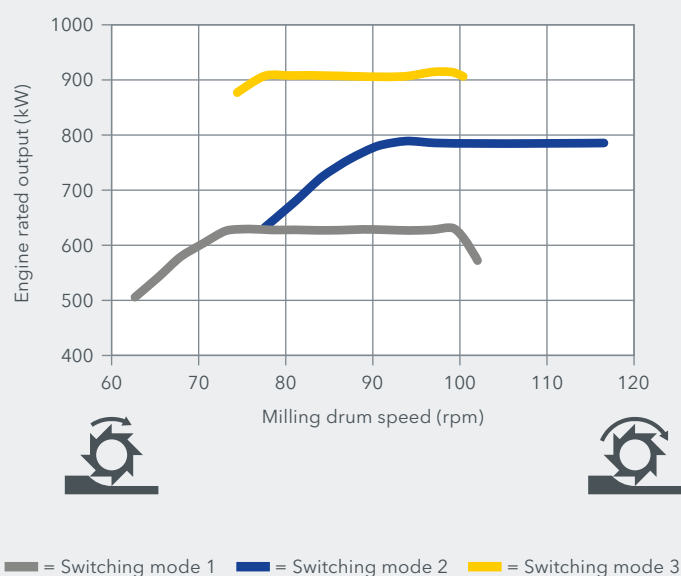
Engine characteristics of the cold milling machine W 250 XF
